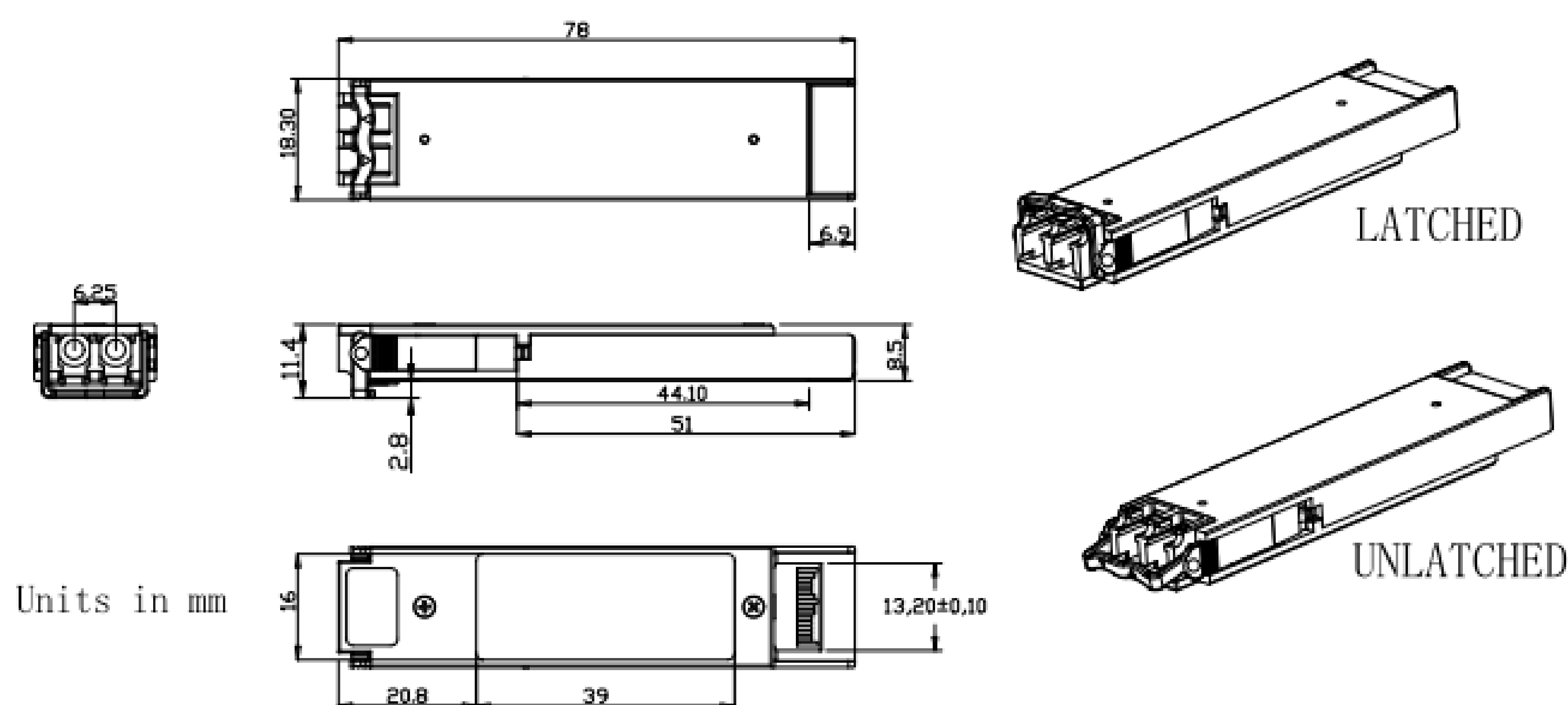
XFP Transceiver (dimensions are in mm)
